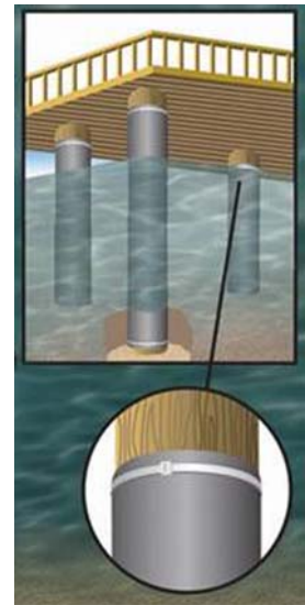
Pier Pilings
